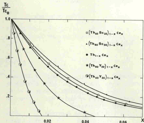
FIGURE 7 T_c/T_{c0} versus Ce concentration c in (Th_{1-x}Y_x)_{1-c}Ce_c and in (Th_{1-x}Sc_x)_{1-c}Ce_c alloys (reference 8).
